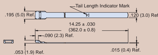
Extended Length Micro-Band 600-083 Precoiled Micro-Band 600-083-1
