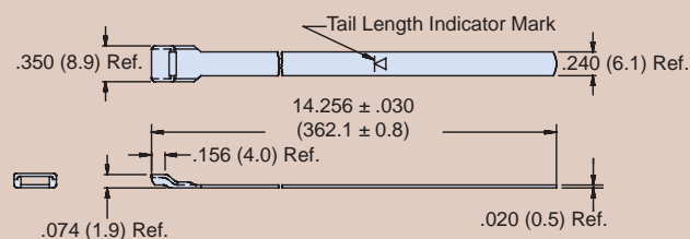
Standard Band 600-052 Precoiled Standard Band 600-052-1
