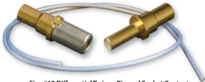
Size #12 Differential Twinax Pin and Socket Contacts and High-Speed Differential Pair Cable
