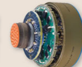
EMP Diode-Equipped Connector with Oversized Shell
