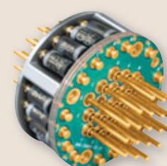
EMI Filter Package with TVS EMP Diodes
