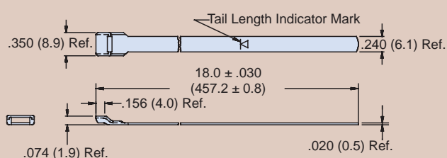
Extended-Length Standard Band 600-090 Precoiled Extended-Length Standard Band 600-090-1
