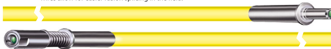
Factory terminated lens pin terminus and lens socket terminus on pigtail wires allow for easier fusion splicing in the field.
